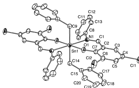
Figure 3. Molecular structure of compound 2 . Thermal ellipsoids are drawn at 30% probability level. Hydrogen atoms have been omitted for clarity.
