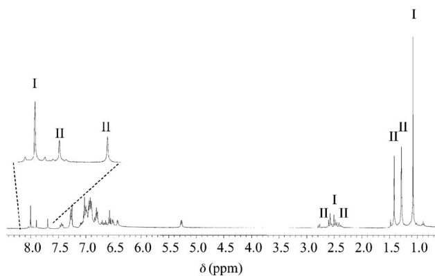
Figure 1. ^1H NMR spectrum ( CDCl_3 , 298 K) of compound 3 .
