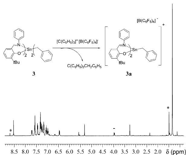
Figure 4. ^1H NMR spectrum ( CD_2Cl_2 , 298 K) of compound 3a : (*) “free” ligand impurities; (■) C(C_6H_5)_3CH_2C_6H_5 .
