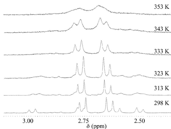
Figure 2. ^1H NMR spectra of aliphatic regions of compound 3 at variable temperature ( ClC_6D_5 ).
