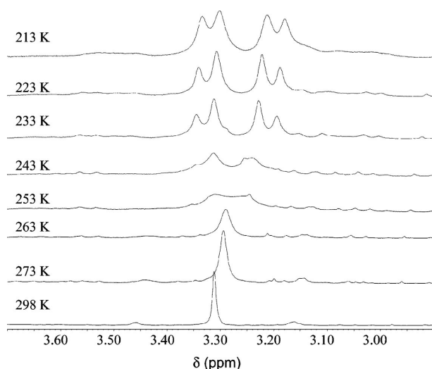
Figure 5. ^1\text{H} NMR spectra of aliphatic region of compound 3a at variable temperature ( \text{CD}_2\text{Cl}_2 ).
